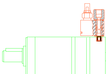
Side Port
