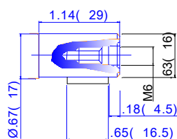
Metric Shaft
