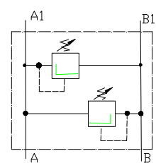
Crossover relief valve CV-XXXX
