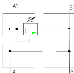
Single Crossover relief valve CV-XXXX-B
