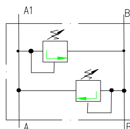
Double Crossover relief valve CV-XXXX
